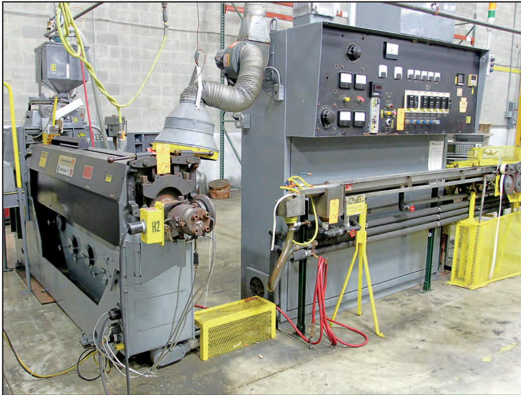
DAVIS STANDARD 350S 3.5" 24:1 EXTRUDER
