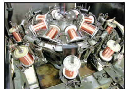
WARDWELL BRAIDER (INTERIOR VIEW)
